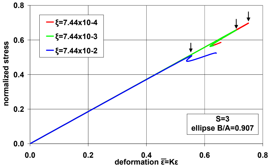
Fig. 27 Load-displacement path for an imperfect elliptic cylinder; arrows (↓) indicate maximum load points ( B/A=0.907 , r_0/t=190 , S=3 )
