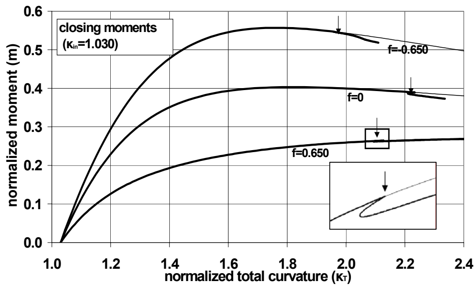
Fig. 62 Numerical results of the response of an initially bent cylinder under closing moments ( \kappa_{in}=1.030 ) for three different levels of pressure f ( r/t=120 ); thick lines correspond to paths with buckling and thin lines to uniform ovalization paths respectively whereas arrows ( \downarrow ) denote bifurcation
