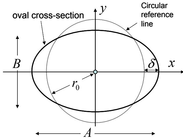
Fig. 16 Non-circular elliptic geometry
