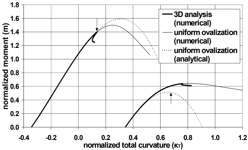
Fig. 77 Comparison of numerical results and analytical solutions for non-pressurized cylinders ( r/t=120 ) and for two different values of initial curvature ( \kappa_{in}=\pm 0.343 ); arrows ( \downarrow \uparrow ) denote the critical points obtained from the analytical solution
