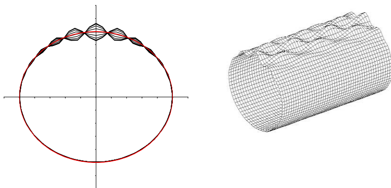
Fig. 94 Buckling modes for a thin cylinder r/t=10 , higher values of anisotropy parameter S result in greater variation in the hoop direction
