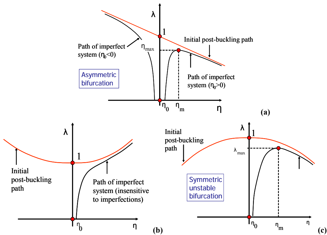
Fig. 108 Load-deflection curves for the post-buckling path (a) a \neq 0 , (b) a=0, b>0 and (c) a=0, b<0 .
