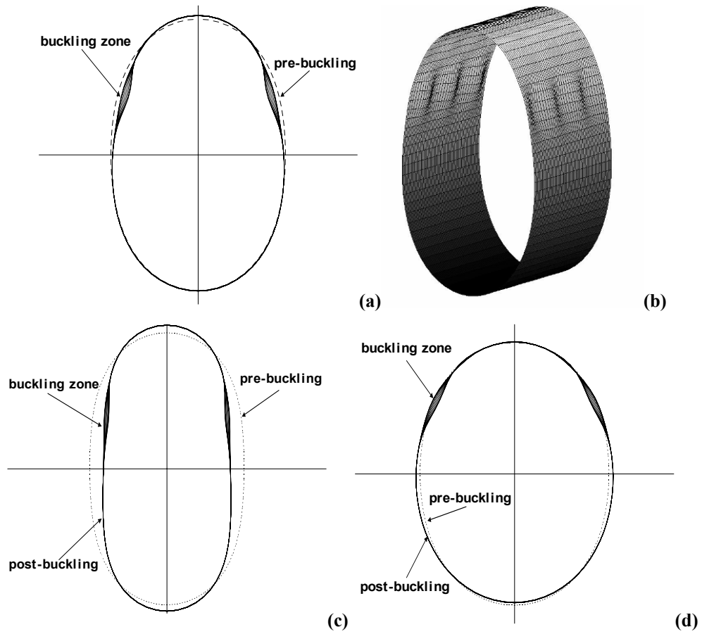
Fig. 68 Pre-buckling and post-buckling shapes; (a) and (b) f=0 , critical point at \theta \approx \pi/6 , (c) f=0.5 , critical point at \theta \approx \pi/6 , (d) f=-0.5 , critical point at \theta \approx 40^\circ ; ( \kappa_m = -1.374 , r/t=120 ).
