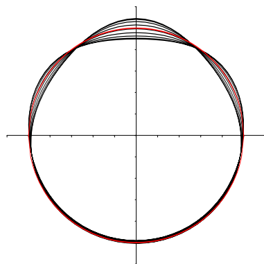
Fig. 93 Buckling modes for a thick cylinder ( r/t=10 ); higher values of anisotropy parameter S result in greater variation in the hoop direction
