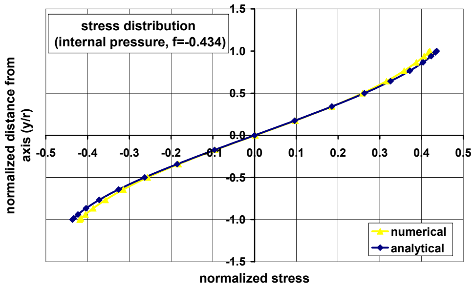
Fig. 42 Longitudinal stress distributions at the ovalization limit point for pressurized bending ( r/t=120, \kappa_{in}=0 )
