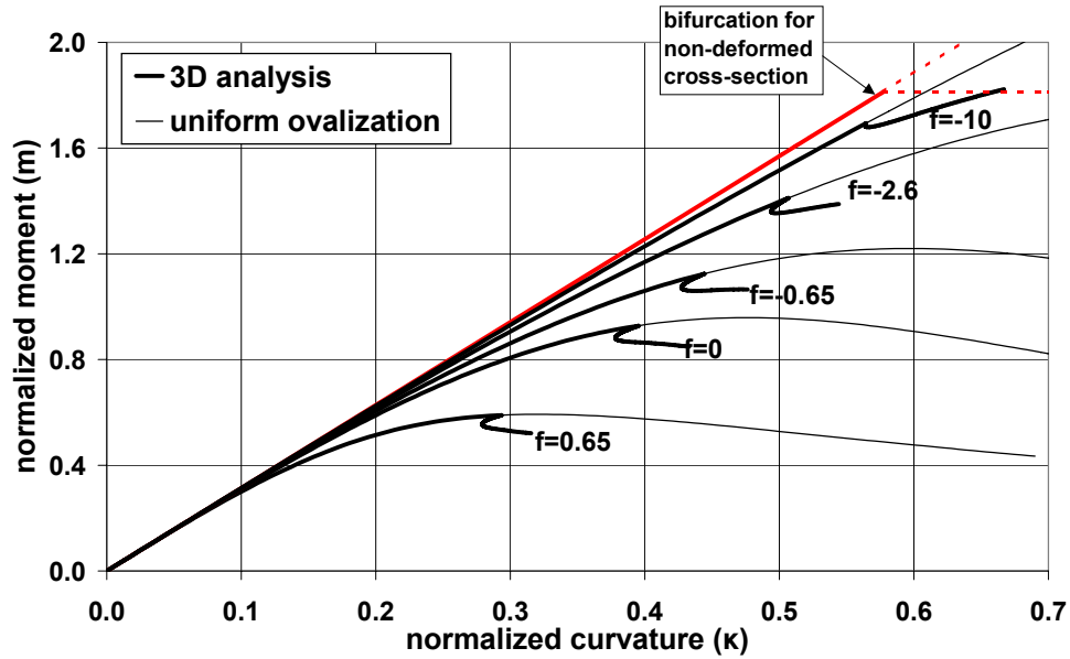
Fig. 52 Numerical results of m - \kappa paths with respect to the level of pressure ( \kappa_{in}=0 , r/t=120 )
