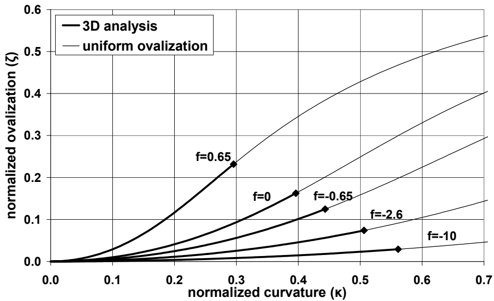
Fig. 53 Numerical results of \zeta - \kappa paths with respect to the level of pressure; points (♦) define bifurcation points numerically calculated ( \kappa_{in}=0 , r/t=120 )
