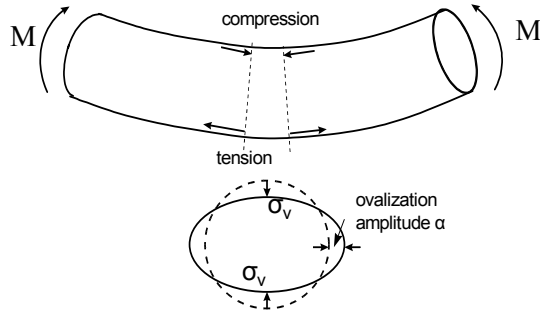
Fig. 32 Ovalization mechanism
