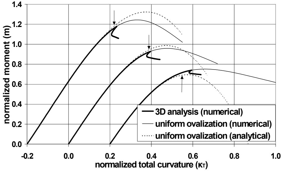
Fig. 76 Comparison of numerical results and analytical solutions for non-pressurized cylinders ( r/t=120 ) and for three different values of initial curvature ( \kappa_{in}=0, \kappa_{in}=\pm 0.2 ); arrows ( \downarrow \uparrow ) denote the critical points obtained from the analytical solution.
